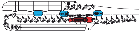
Launch / recovery area separated by the island Single Island / 3 x Internal lifts
