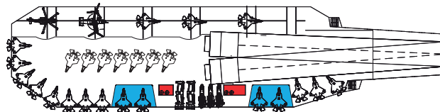
Converging twin runways Split Island / deck-edge lifts (Starboard)
